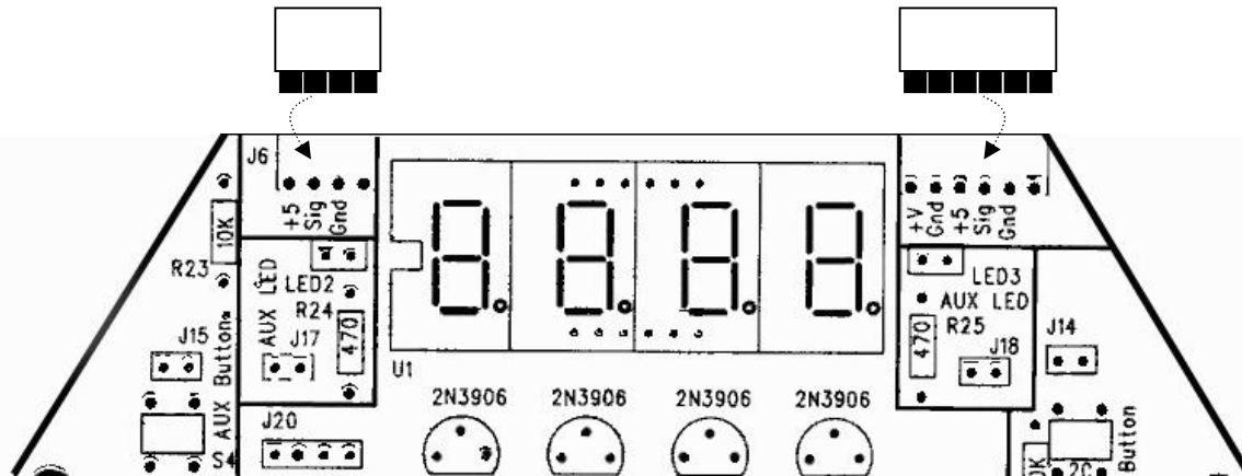
Figure 3-5: 4-pin and 6-pin edge connectors (for bumper switch attachment).
