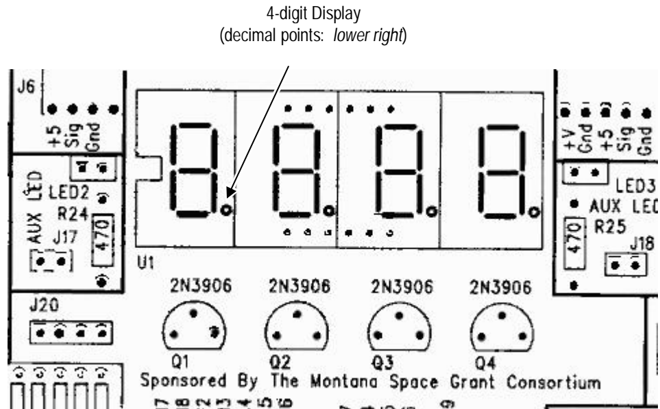
Figure 3-1: Position of 4-digit LED Display
